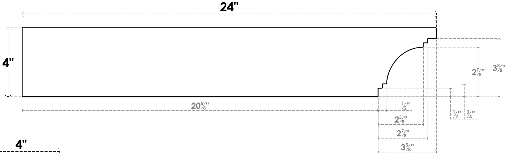
SIDE PROFILE
